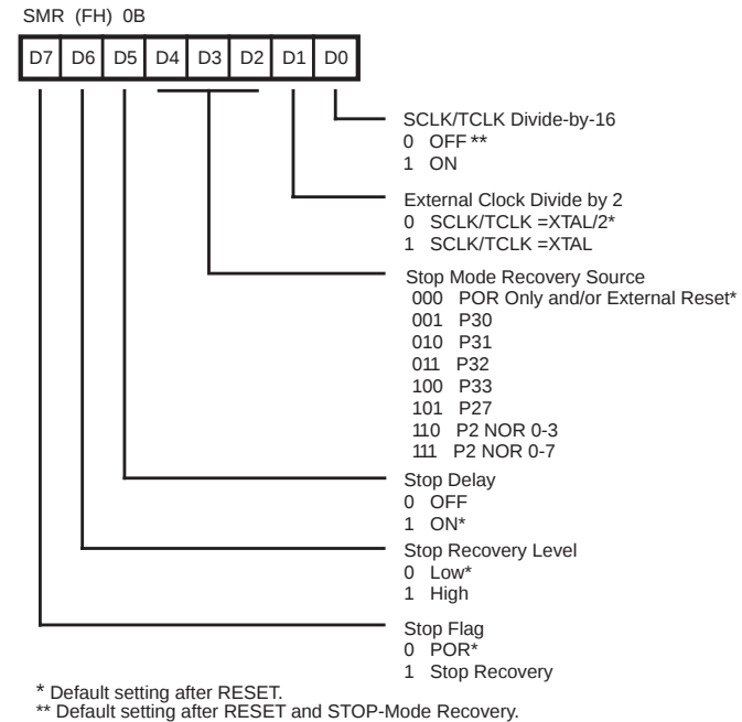
Figure 42. STOP-Mode Recovery Register Write Only Except Bit D7, Which is Read Only
