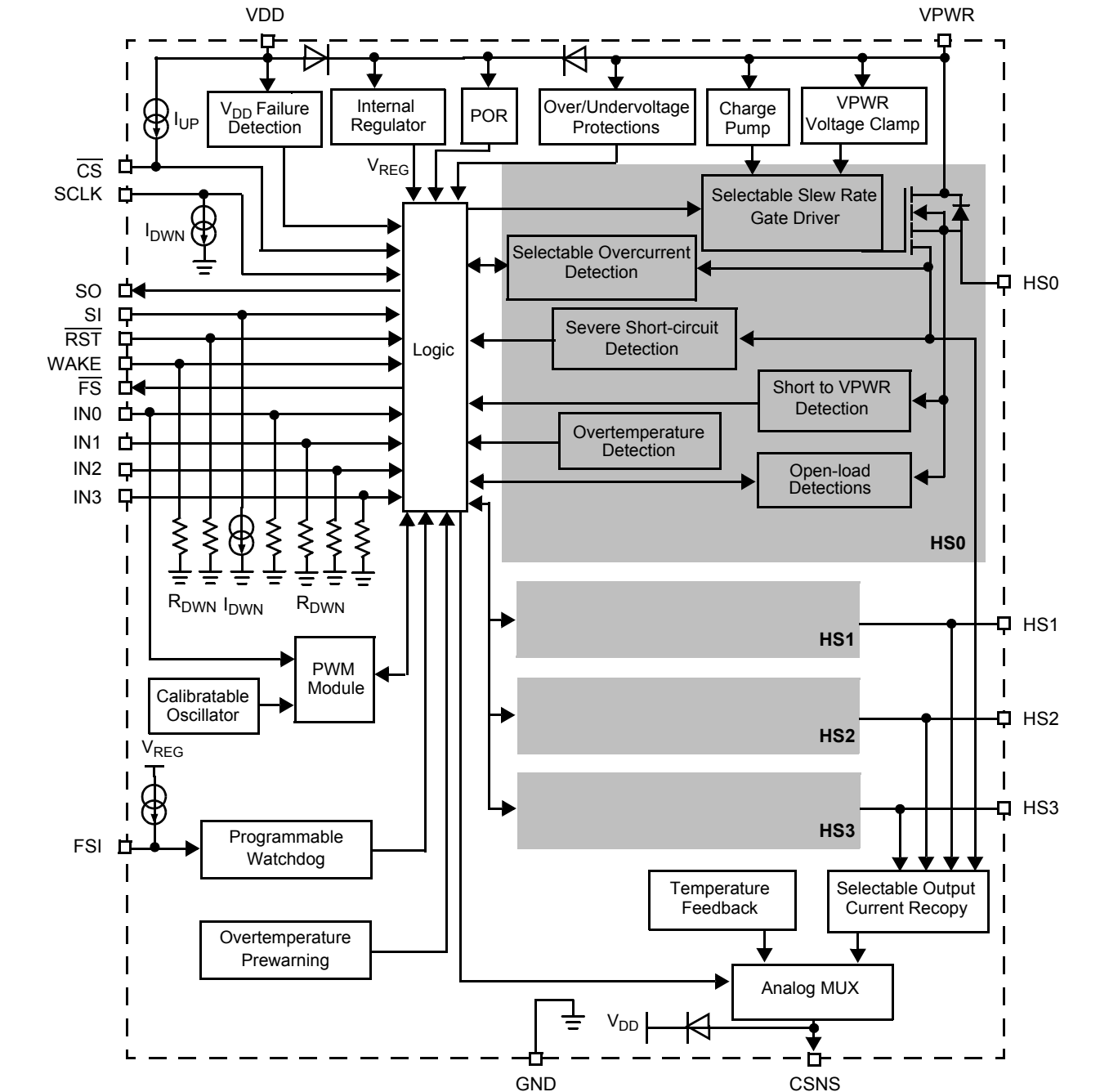
Figure 2. 10XS3412 Simplified Internal Block Diagram
