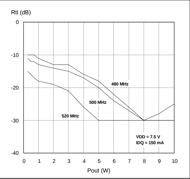
Figure 9. Return loss vs. output power
