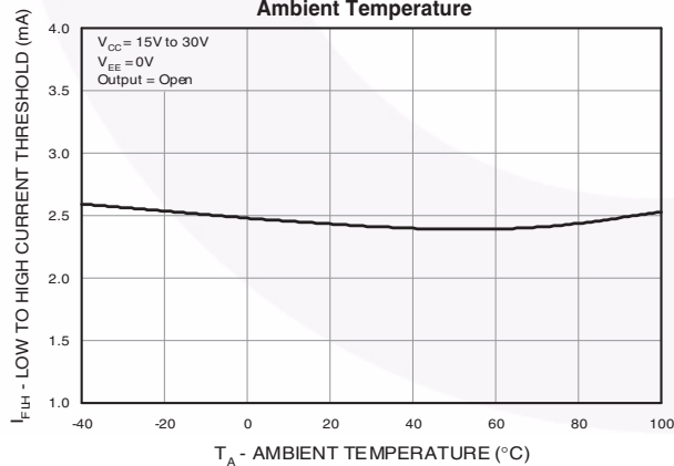
Fig. 11 Low to High Input Current Threshold vs. Ambient Temperature
