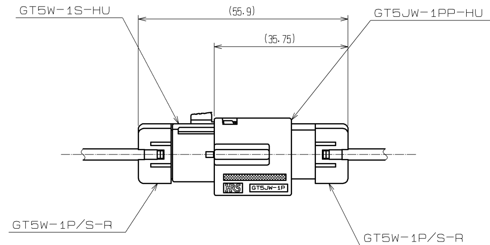
MATED CONNECTORS
