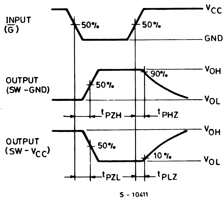
WAVEFORM 2: OUTPUT ENABLE AND DISABLE TIMES ( f=1\text{MHz} ; 50% duty cycle)
