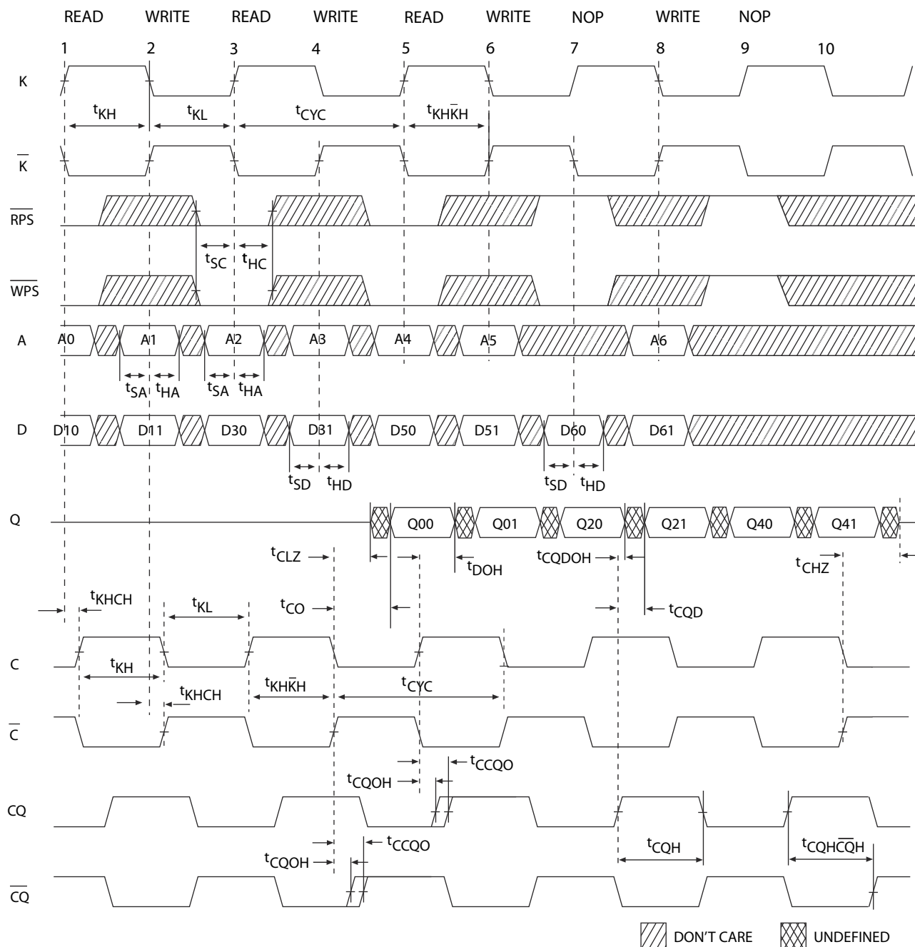
Figure 6. Read/Write/Deselect Sequence [36, 37, 38]
