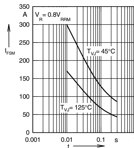
Fig. 1 Non-repetitive peak surge current (Rectifier Diodes)
