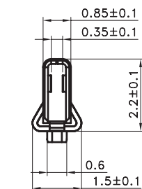
SEC.C-C
