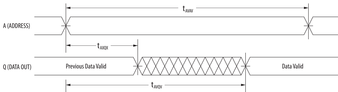
Figure 6 – Read Cycle 1
