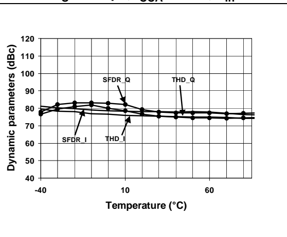
Figure 10. Distortion vs. Temperature F_S=20\text{Msps} ; I_{CCA}=40\text{mA} ; F_{in}=2\text{MHz}
