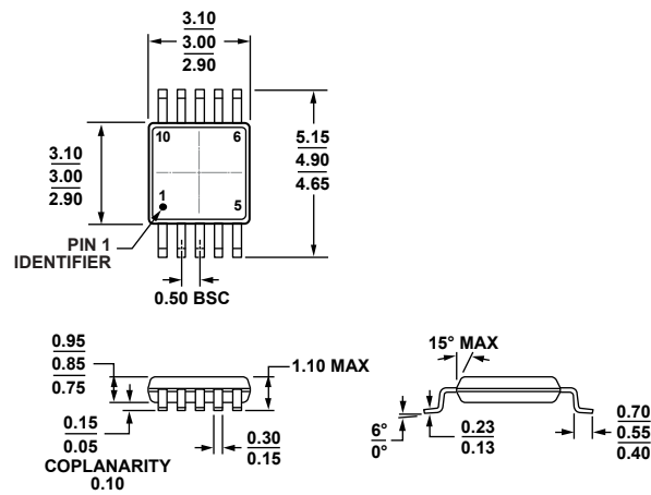
COMPLIANT TO JEDEC STANDARDS MO-187-BA Figure 32. 10-Lead Mini Small Outline Package [MSOP] (RM-10)
