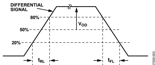
Figure 2. LVDS Timing, Differential
