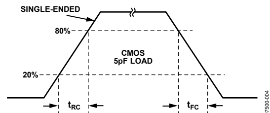
Figure 3. LVCMOS Timing
