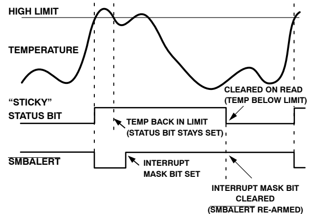
Figure 25. How Masking the Interrupt Source Affects SMBALERT Output
