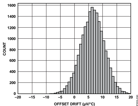
Figure 25. Offset Drift
