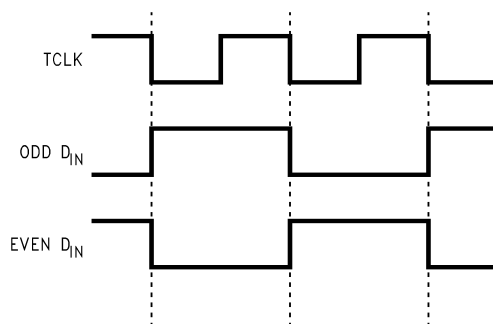
Figure 1. "Worst Case" Serializer IDD Test Pattern
