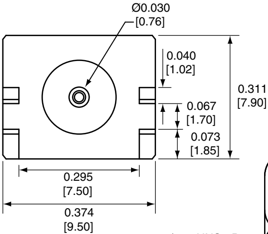
BACK VIEW
