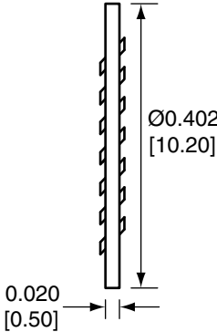
RECOMMENDED MOUNTING HOLE
