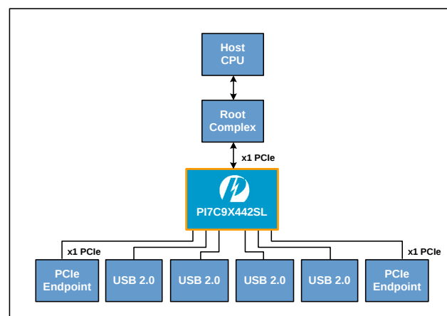
PI7C9X442SL – Block Diagram
