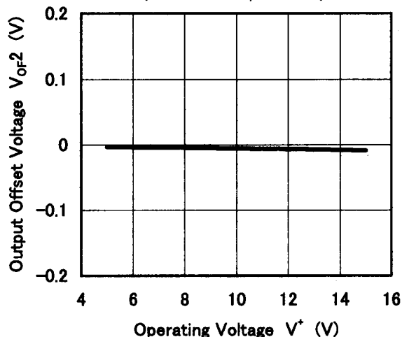
Output Offset Voltage vs. Operating Voltage (OUT1-OUT2, T_a=25^\circ\text{C} )
