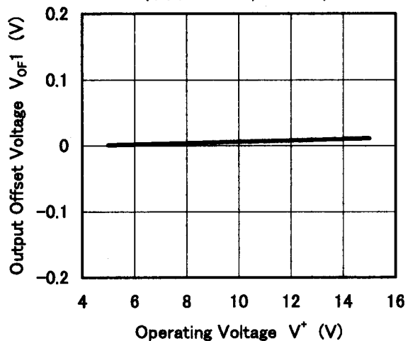
Output Offset Voltage vs. Operating Voltage (OUT3-OUT4, T_a=25^\circ\text{C} )
