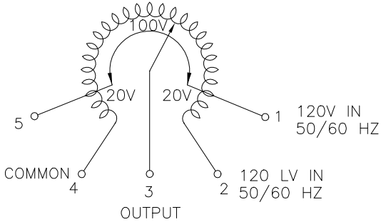
SCHEMATIC VIEW FROM BASE END
