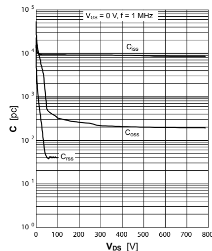
Fig. 9 Typ. capacitances
