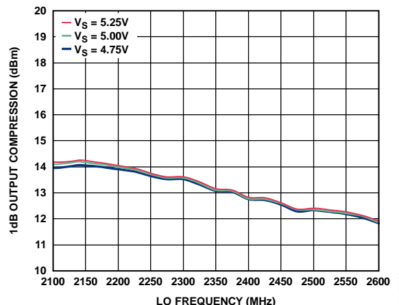
Figure 8. SSB Output 1dB Compression Point ( \text{OP1dB} ) vs. LO Frequency ( f_{\text{LO}} ) and Power Supply
