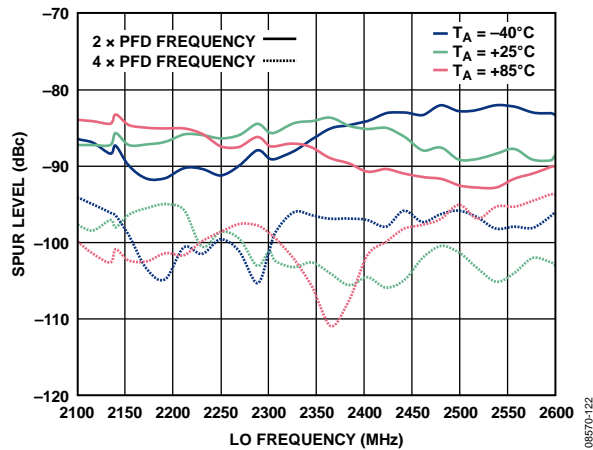
Figure 22. PLL Reference Spurs vs. LO Frequency (2× PFD and 4× PFD) at Modulator Output
