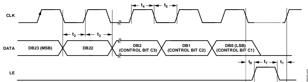
Figure 2. Timing Diagram
