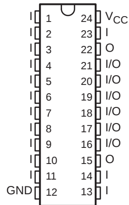
TIBPAL20L8' C SUFFIX . . . JT OR NT PACKAGE M SUFFIX . . . JT PACKAGE
