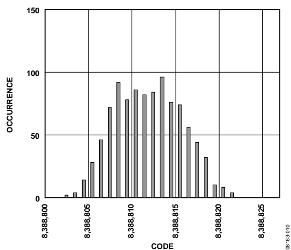
Figure 10. Noise Distribution Histogram ( V_{REF} = AV_{DD} , Output Data Rate = 120 Hz, Gain = 1)
