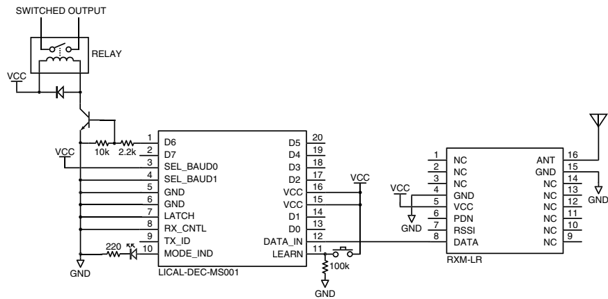
Figure 15: LR Series Receiver and MS Series Decoder
