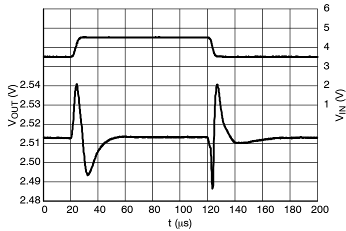
Figure 32. Line Transients, 2.5 V Version, t_R = t_F = 5 \mu s , I_{OUT} = 30 \text{ mA} , C_{OUT} = 100 \text{ nF}
