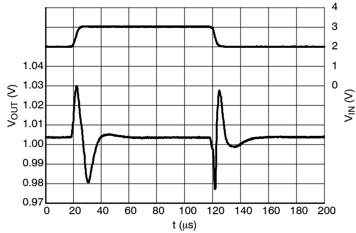
Figure 28. Line Transients, 1.0 V Version, t_R = t_F = 5 \mu s , I_{OUT} = 30 \text{ mA} , C_{OUT} = 100 \text{ nF}
