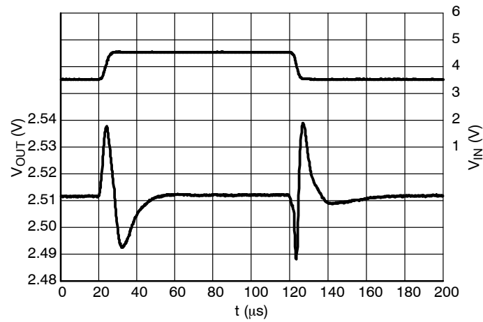
Figure 31. Line Transients, 2.5 V Version, t_R = t_F = 5 \mu s , I_{OUT} = 30 \text{ mA} , C_{OUT} = 0 \text{ nF}
