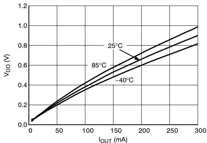
Figure 6. Dropout Voltage vs. Output Current 1.0 V Version
