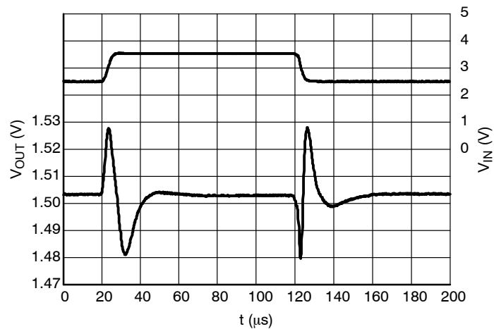
Figure 29. Line Transients, 1.5 V Version, t_R = t_F = 5 \mu s , I_{OUT} = 30 \text{ mA} , C_{OUT} = 0 \text{ nF}
