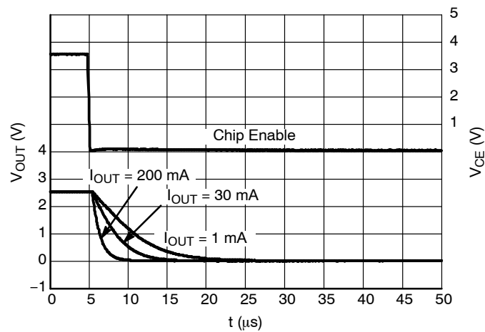
Figure 44. Shutdown, 2.5 V Version D, V_{IN} = 3.5 \text{ V}
