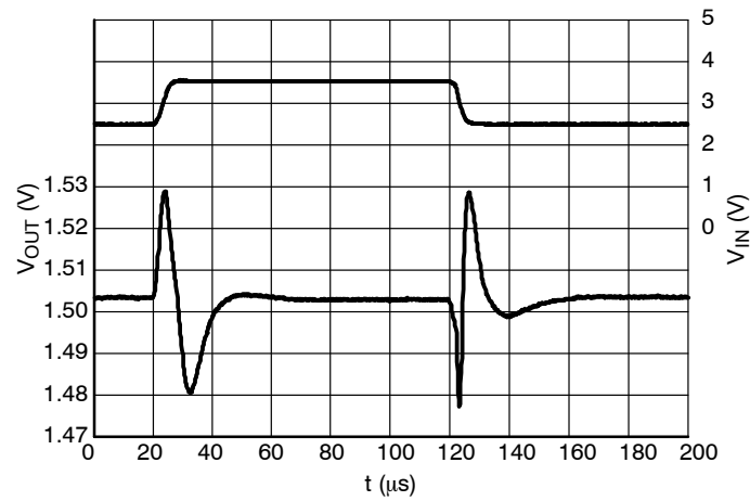
Figure 30. Line Transients, 2.5 V Version, t_R = t_F = 5 \mu s , I_{OUT} = 30 \text{ mA} , C_{OUT} = 100 \text{ nF}
