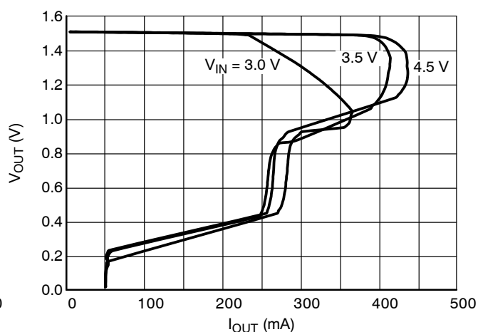
Figure 4. Output Voltage vs. Output Current 1.5 V Version ( T_A = 25^\circ\text{C} )
