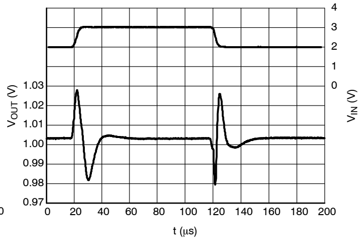
Figure 27. Line Transients, 1.0 V Version, t_R = t_F = 5 \mu s , I_{OUT} = 30 \text{ mA} , C_{OUT} = 0 \text{ nF}
