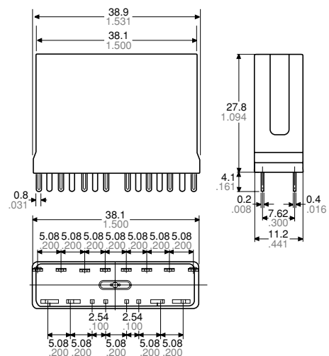
External dimensions
