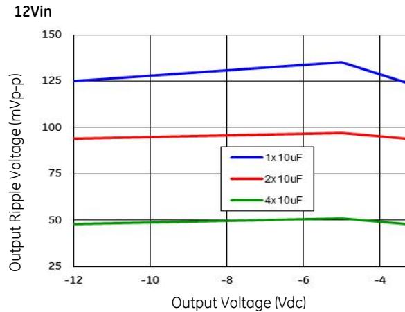
Figure 63. Output ripple with 1x10 \mu F, 2x10 \mu F & 4x10 \mu F output ceramic capacitors (max load).
