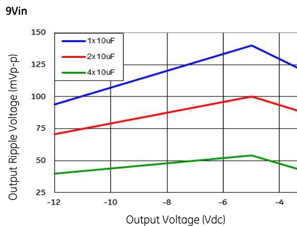
Figure 62. Output ripple with 1x10 \mu F, 2x10 \mu F & 4x10 \mu F output ceramic capacitors (max load).
