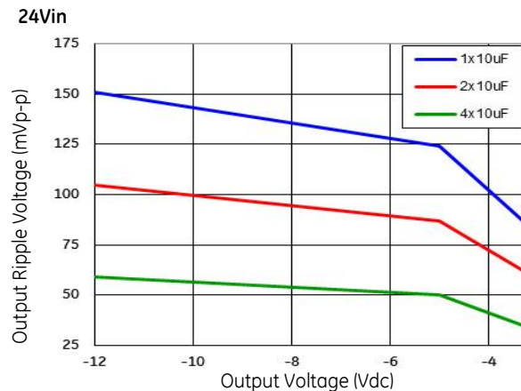
Figure 64. Output ripple with 1x10 \mu F, 2x10 \mu F & 4x10 \mu F output ceramic capacitors (max load).
