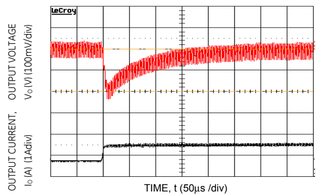
Figure 22. Transient Response to Dynamic Load Change from 50% to 100% at 28Vin, Cext - 1x10uF ceramic, CTune=open & RTune=open
