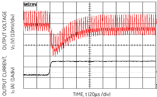
Figure 10. Transient Response to Dynamic Load Change from 50% to 100% at 28V in , C ext = 10μF ceramic + 330μF polymer, C Tune =5600pF & R Tune =261Ω
