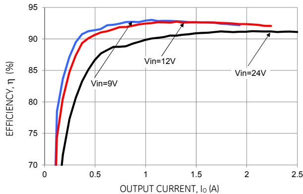
Figure 48. Converter Efficiency versus Output Current.
