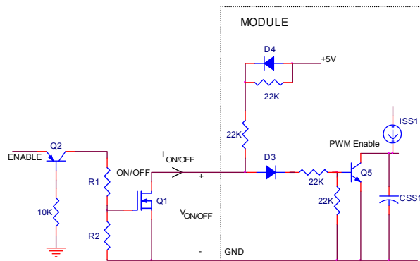
Figure 45. On/Off Level Shifting Circuit for the 3A ProLynx module for negative output applications.
