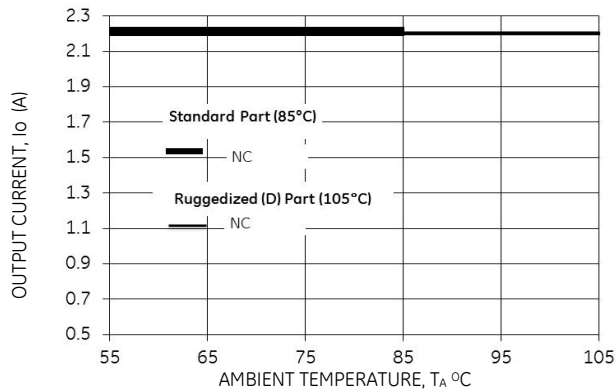
Figure 50. Derating Output Current versus Ambient Temperature and Airflow.
