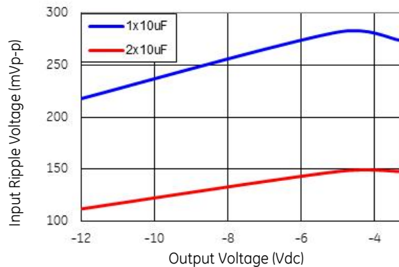
Figure 60. Input ripple voltage with 1x10 \mu F or 2x10 \mu F ceramic capacitors at the input (max load).
