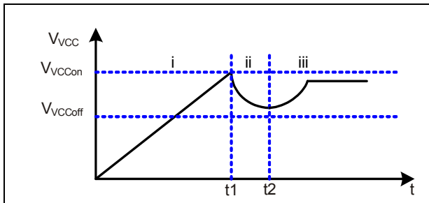
Figure 3 VCC voltage at start up
