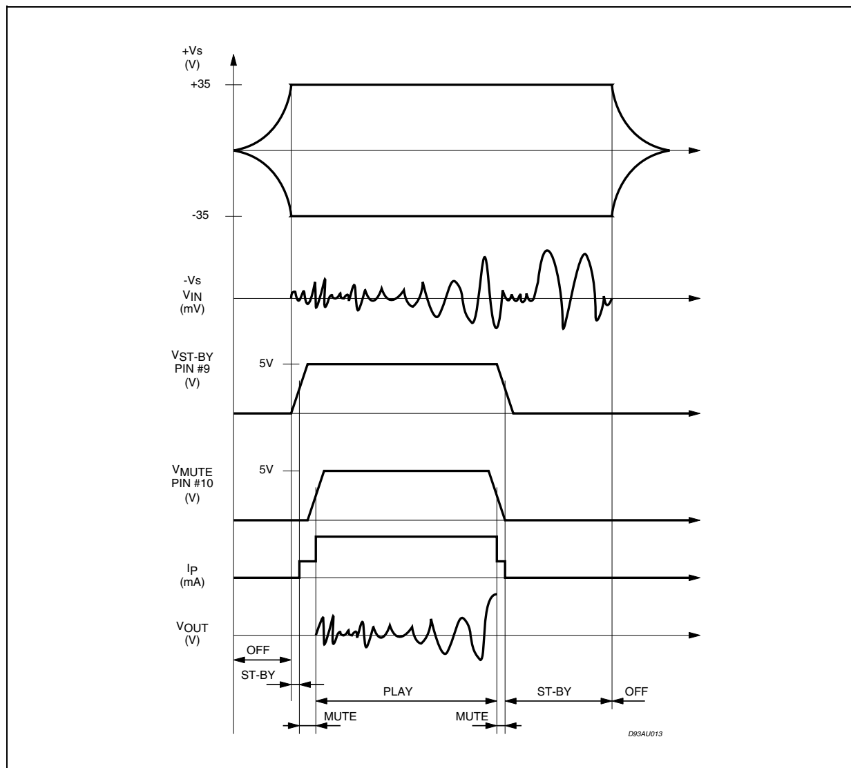
Figure 19. Turn ON/OFF Suggested Sequence
