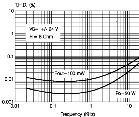
Figure 10. Distortion vs. Frequency
