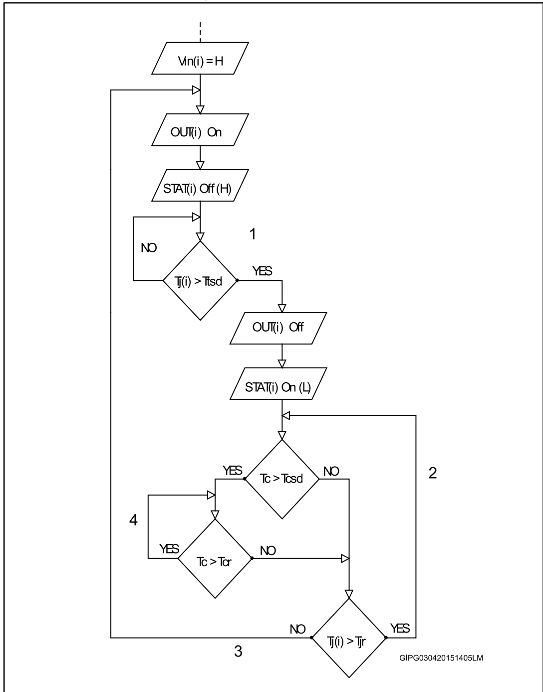
Figure 14: Thermal behavior
