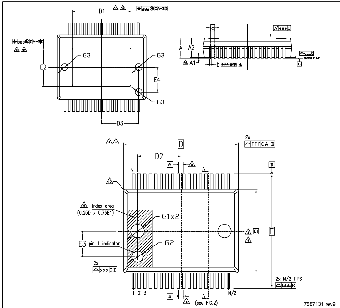
Figure 18: PowerSSO-36 package outline
