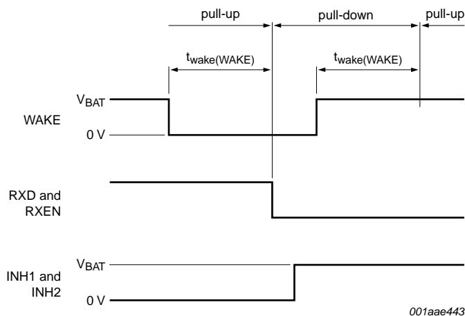
Fig 10. Local wake-up timing via pin WAKE
