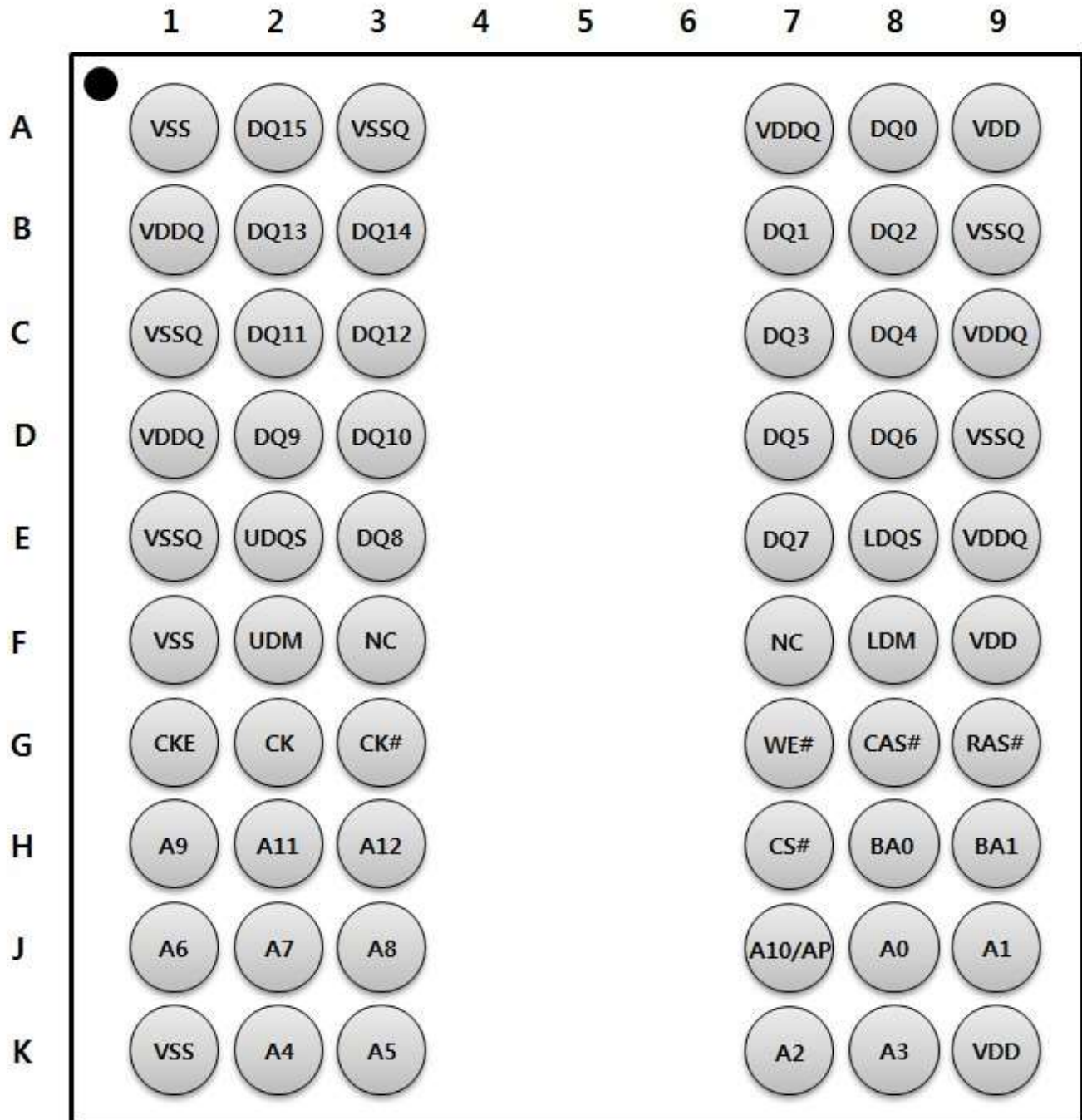
Figure 2.2 Pin configurations
