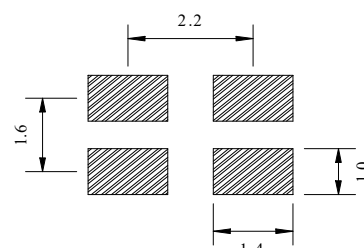
<SUGGESTED LAYOUT>
