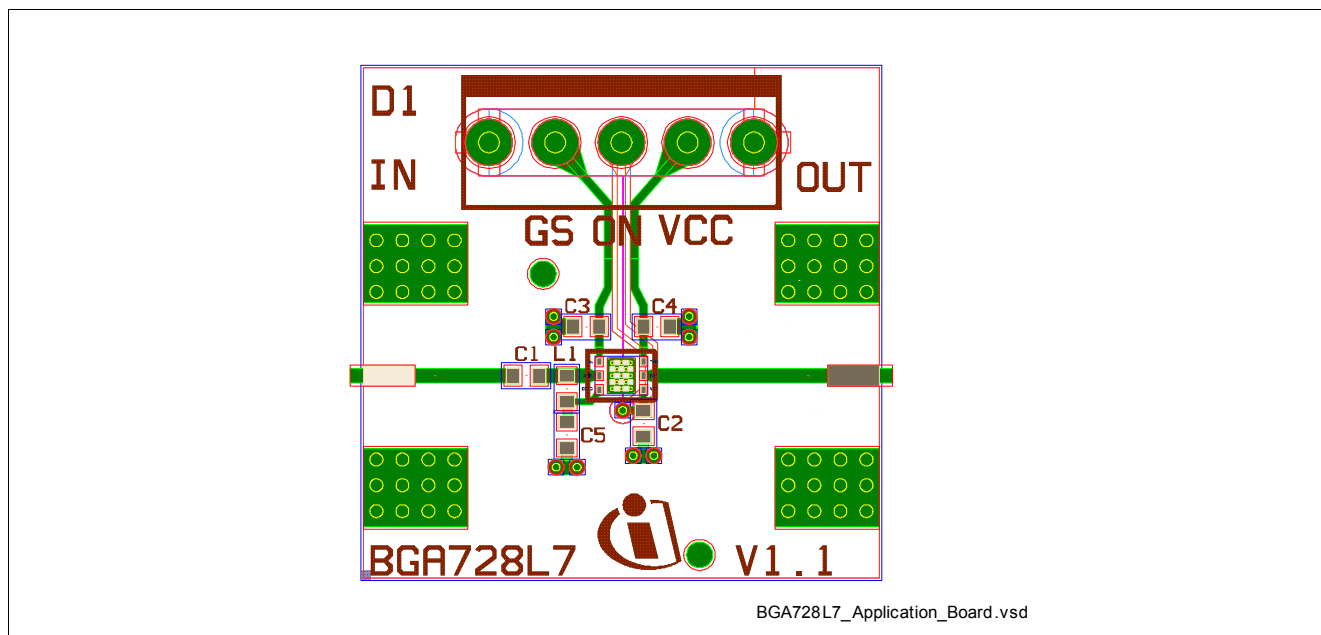
Figure 3 Application Board
