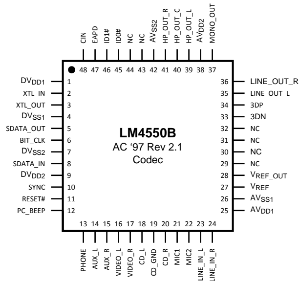
Figure 10. Top View See Package Number PT
