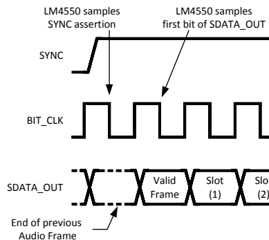
Figure 21. Start of AC Link Output Frame
