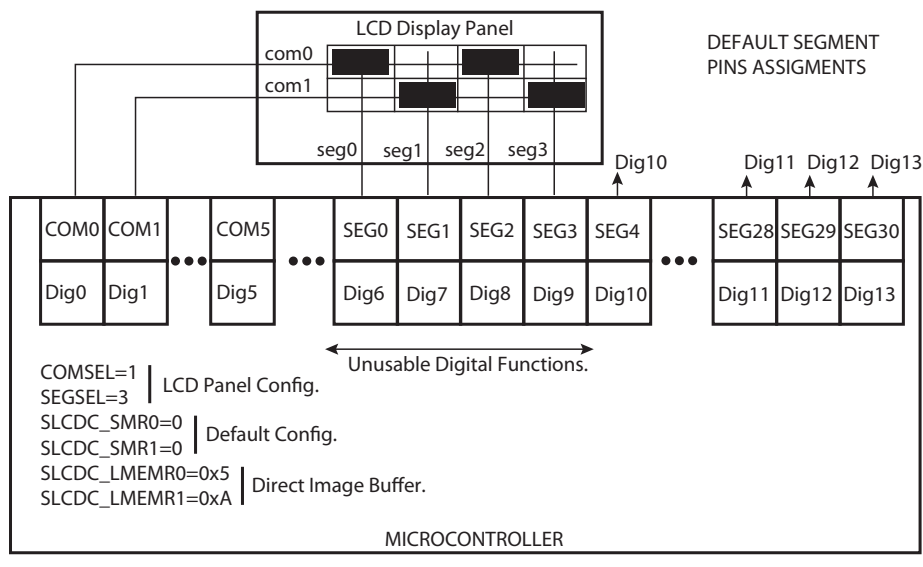
Figure 39-13.Segments Remapping Example
