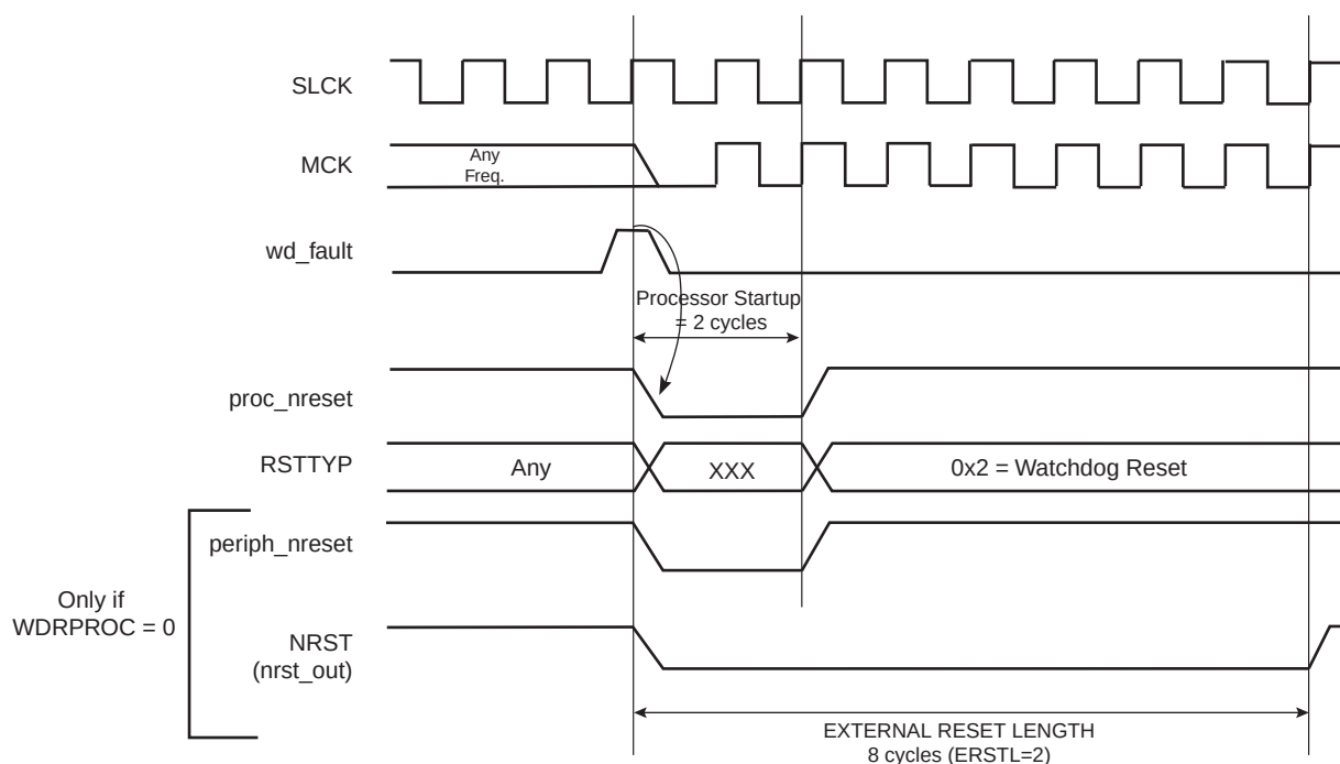
Figure 15-6. Watchdog Reset
