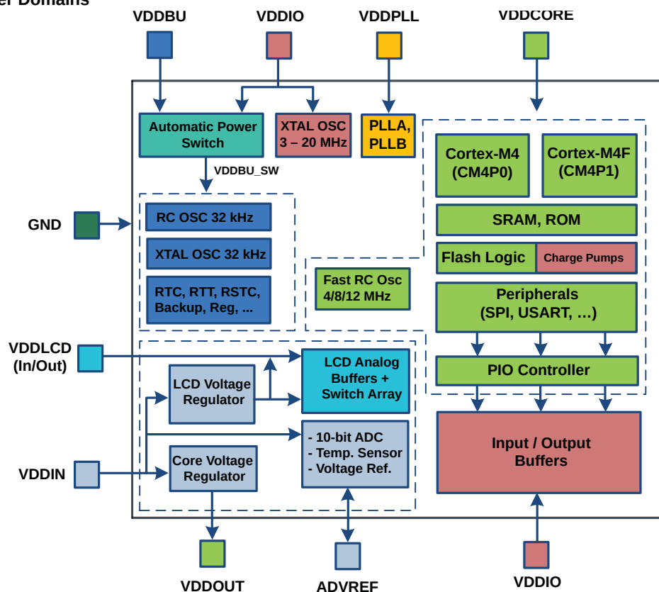
Figure 5-1. Power Domains
