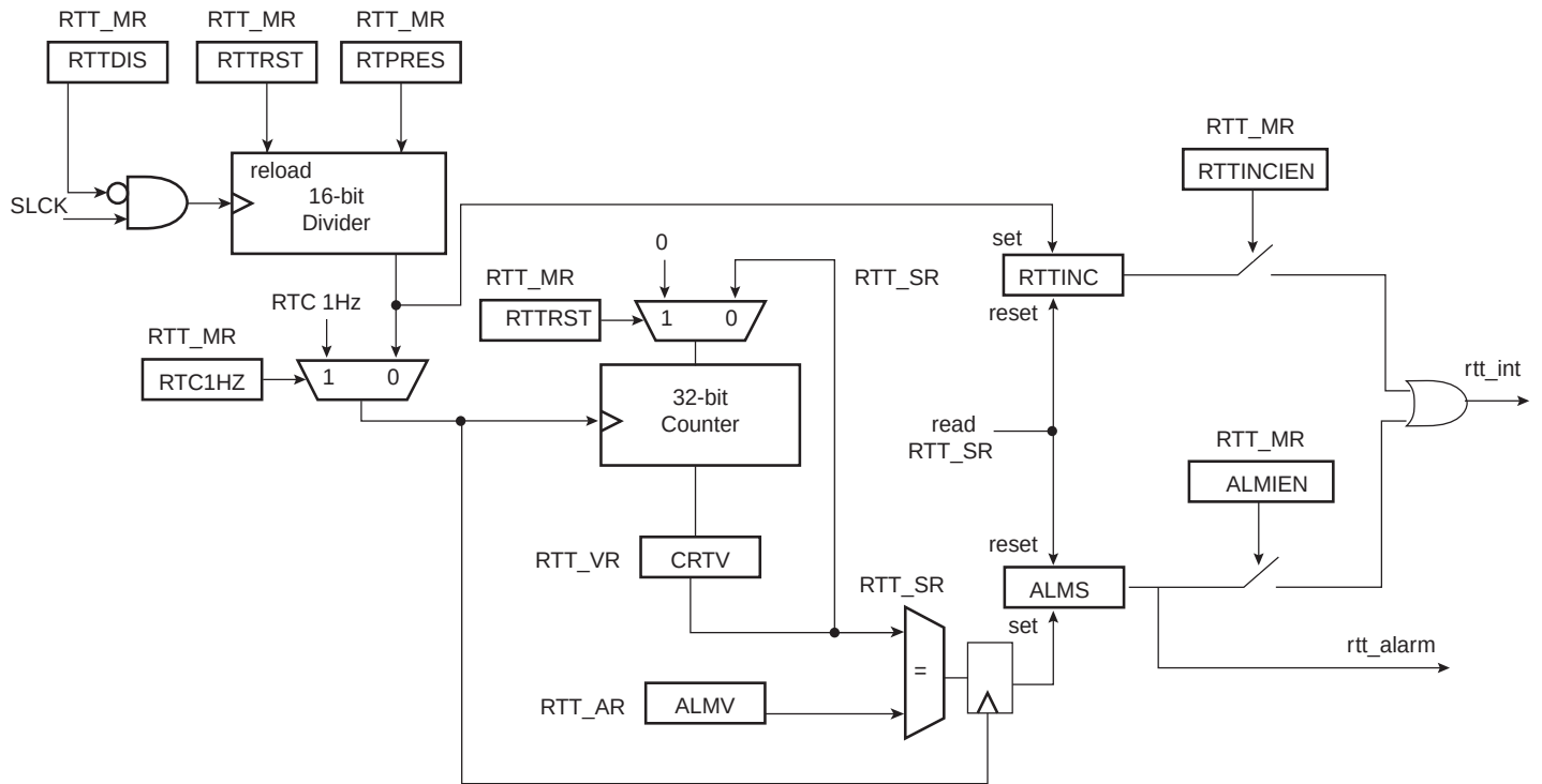
Figure 16-1. Real-time Timer
