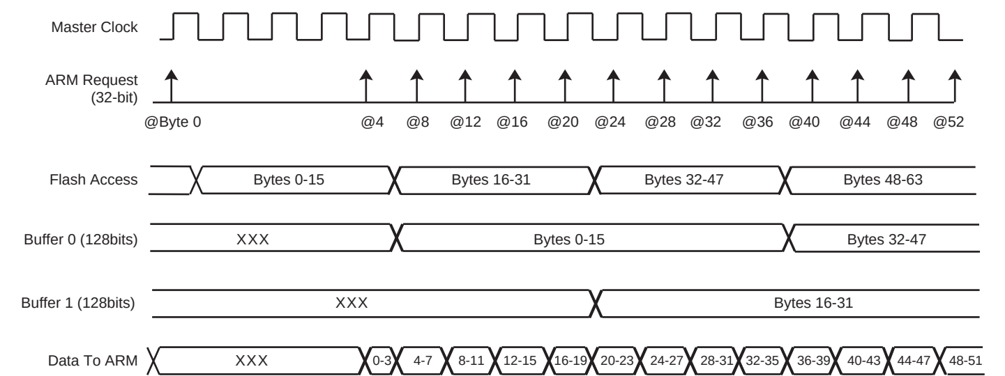
Figure 22-3. Code Read Optimization for FWS = 3
