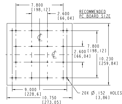
CLHS-625 HANDLE
