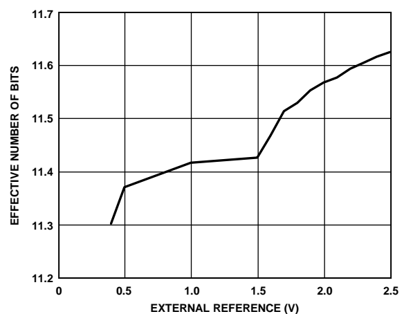
Figure 9. Effective Number of Bits vs. V_{REF} , f_{SCL} = 400 kHz
