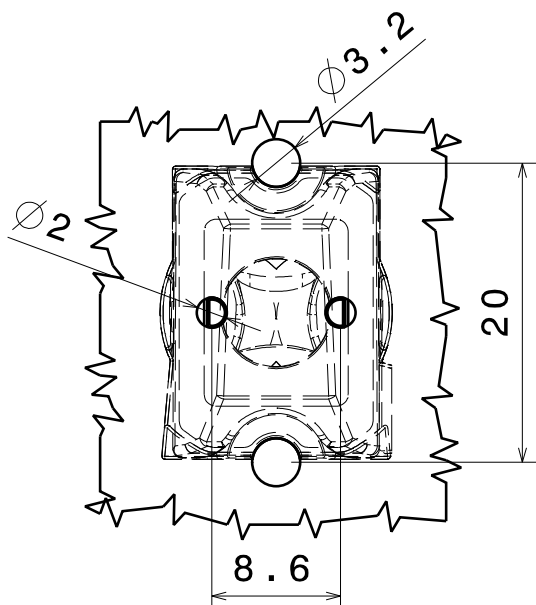
PCB- suggestion
