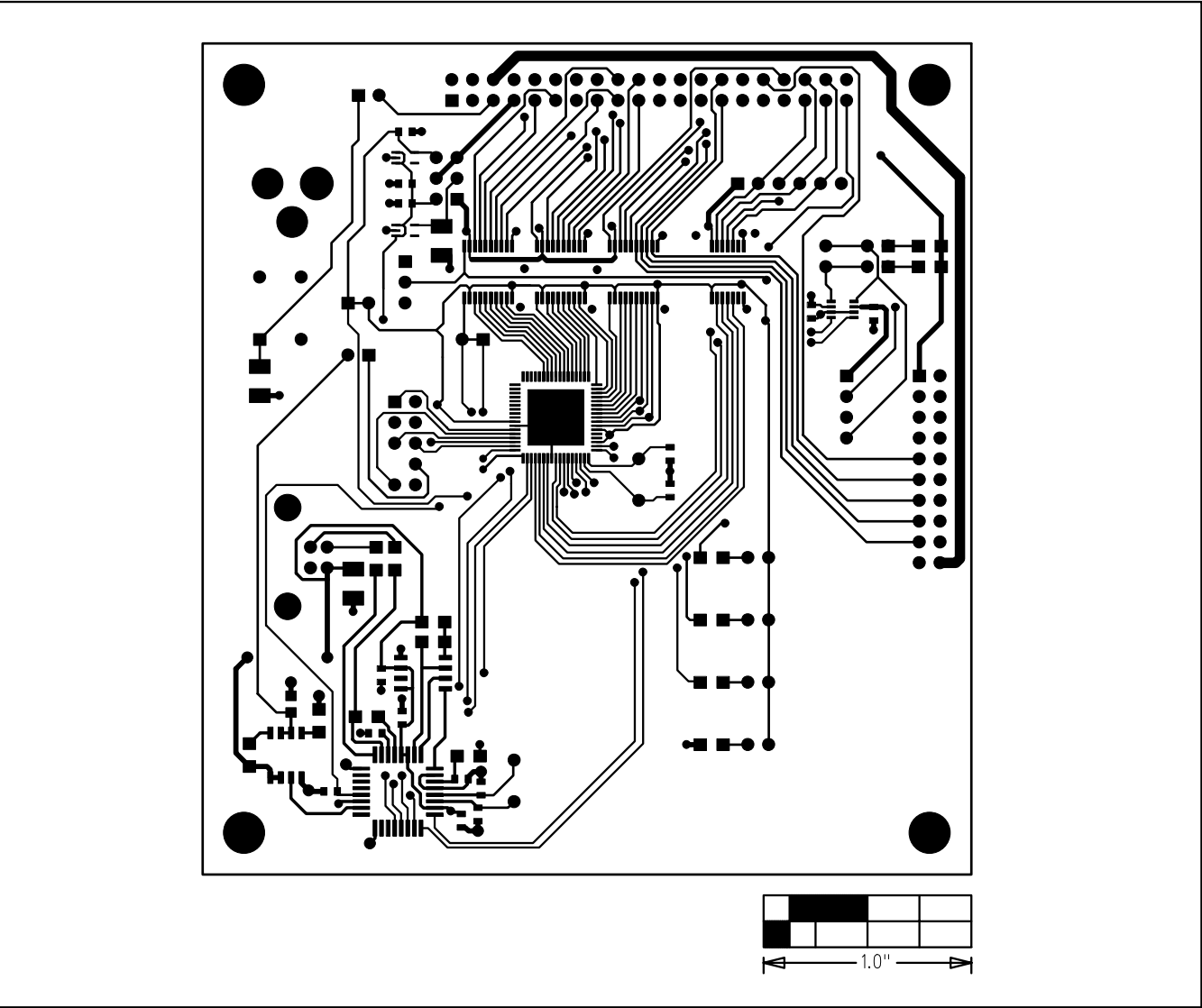
Figure 4. CMAXQUSB PCB Layout—Component Side
