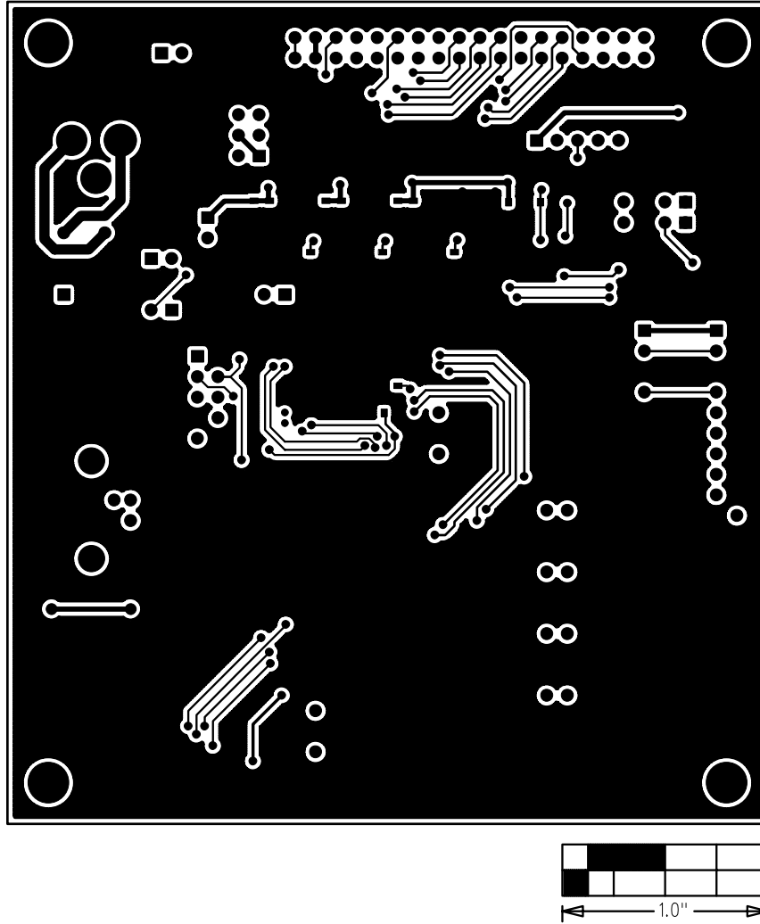
Figure 5. CMAXQUSB PCB Layout—Solder Side
