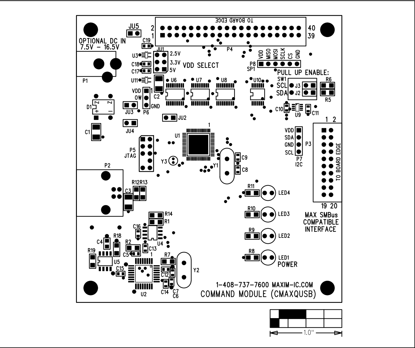
Figure 2. CMAXQUSB Component Placement Guide—Component Side (Top Silkscreen)
