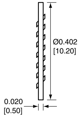
WASHER
