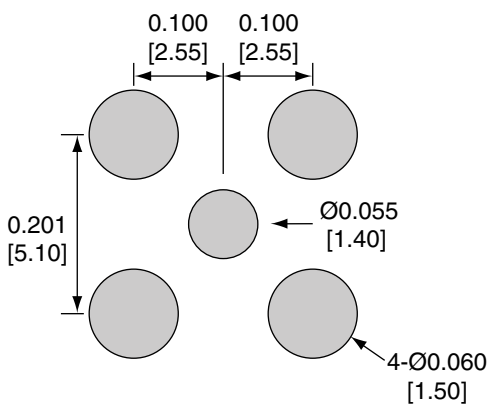
RECOMMENDED FOOTPRINT
