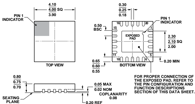
Figure 12. 20-Lead Lead Frame Chip Scale Package [LF CSP_WQ] 4 mm x 4 mm Body, Very Very Thin Quad (CP-20-6)
