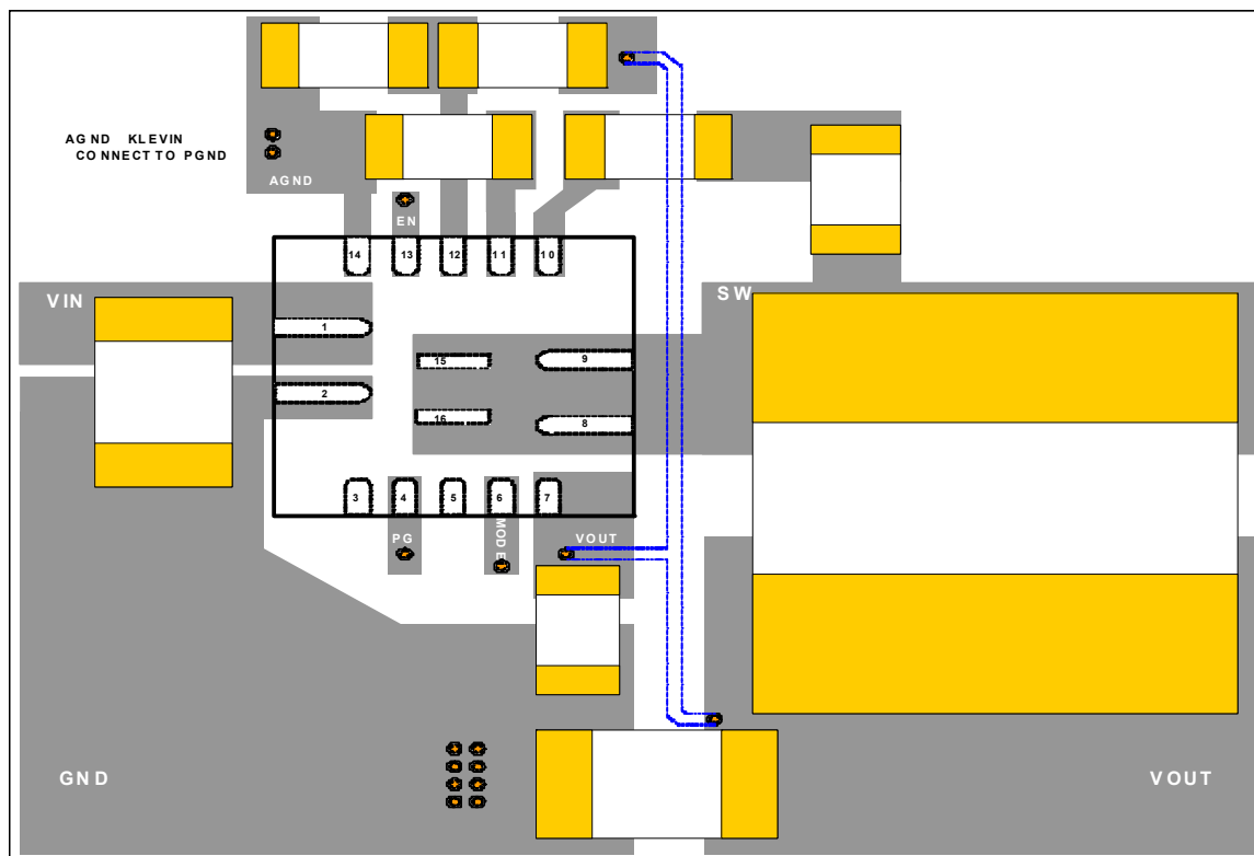
Figure 13—Recommend Layout
