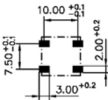
J-lead
