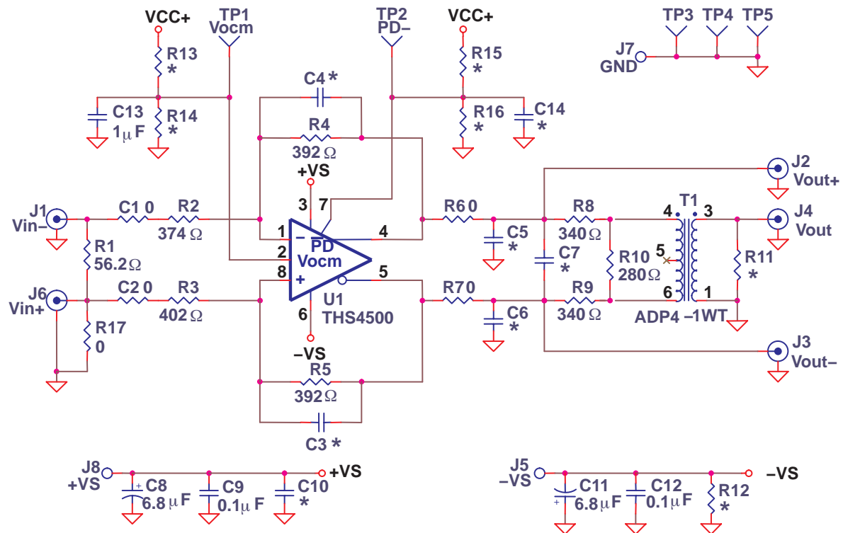
Figure 5–3. Schematic Diagram
