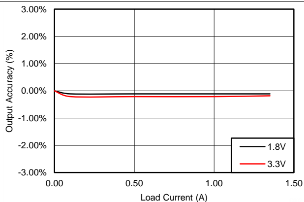
Figure 29. DC-DC Converter - DC Load Regulation Example (Typical)
