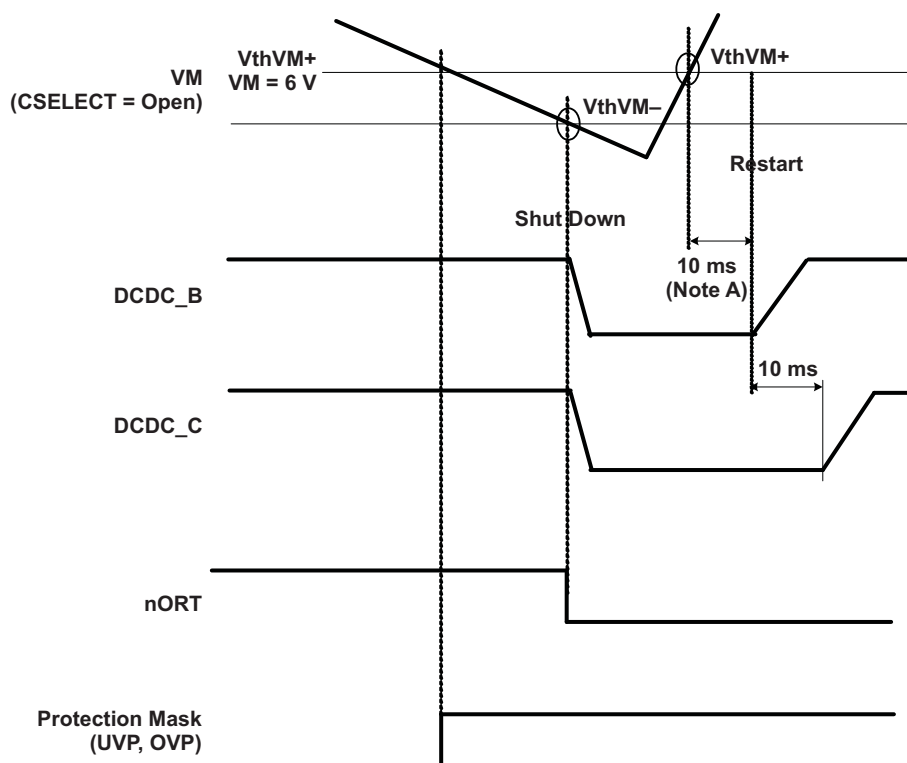
Figure 19. Power-Down Timing (With Glitch on VM Below V_{thVM-} )
