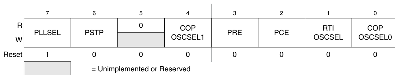
Figure 10-9. S12CPMU Clock Select Register (CPMUCLKS)
