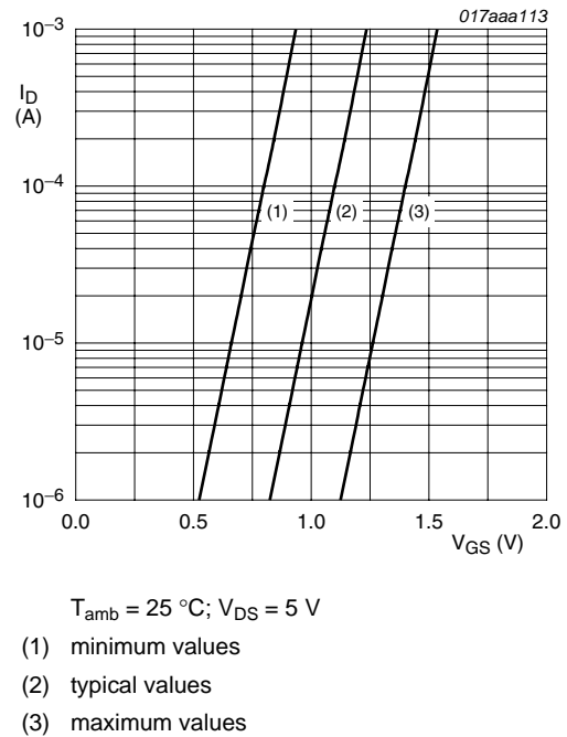
Fig 7. Per transistor: Sub-threshold drain current as a function of gate-source voltage
