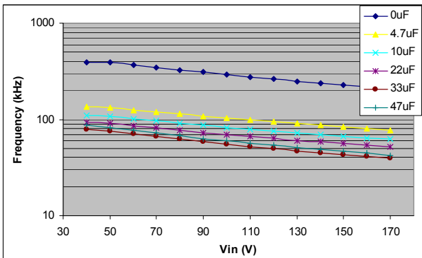
Fig. 13 I_{out} = 350\text{ mA} , V_{out} = 16.8\text{ V} , L = 470\text{ }\mu\text{H}
