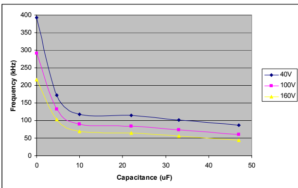
Fig. 14 I_{out} = 350 \text{ mA} , V_{out} = 16.8 \text{ V} , L = 470 \text{ }\mu\text{H}
